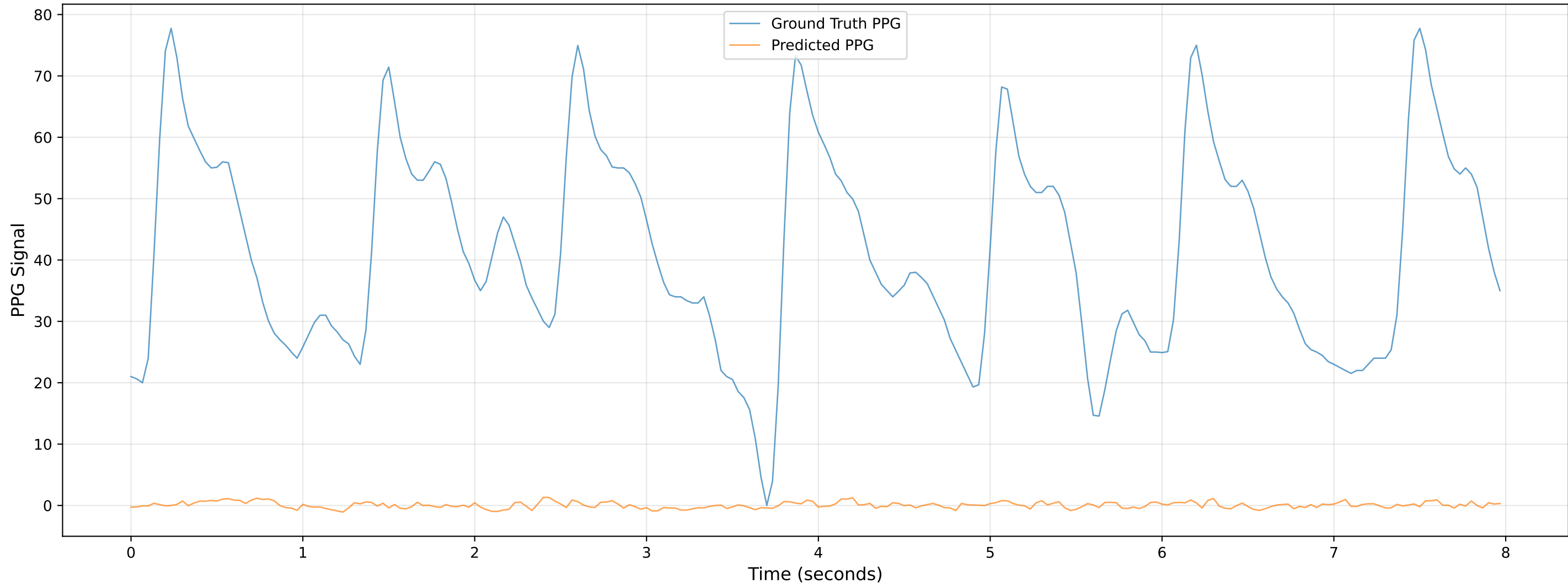
Video 505 - Chunk 4 - Predicted vs Ground Truth PPG
