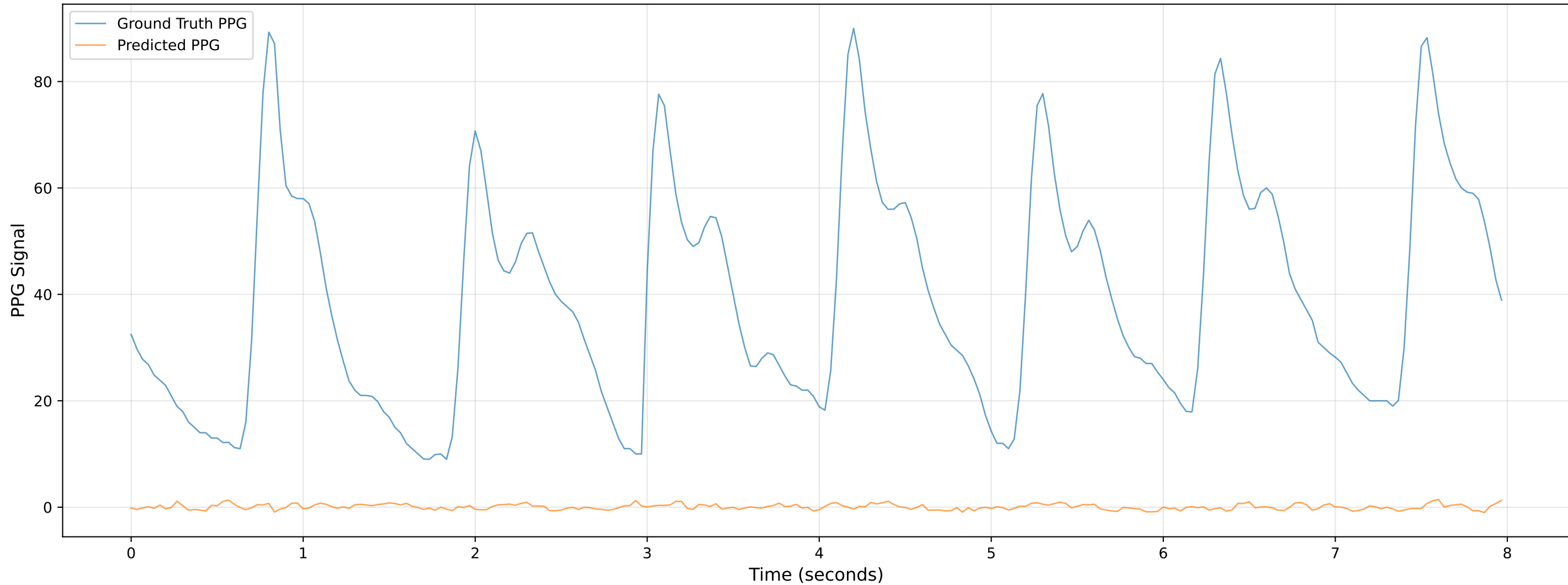
Video 506 - Chunk 3 - Predicted vs Ground Truth PPG
