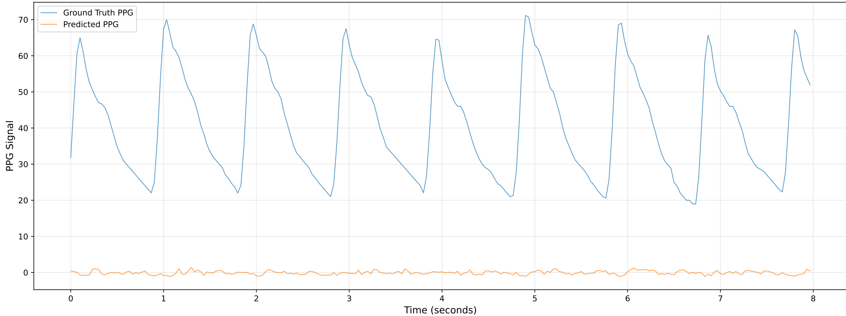
Video 601 - Chunk 3 - Predicted vs Ground Truth PPG
