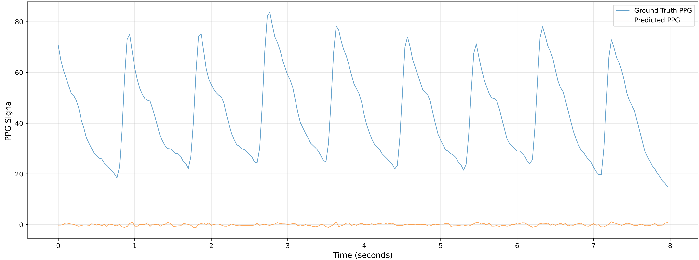
Video 601 - Chunk 6 - Predicted vs Ground Truth PPG
