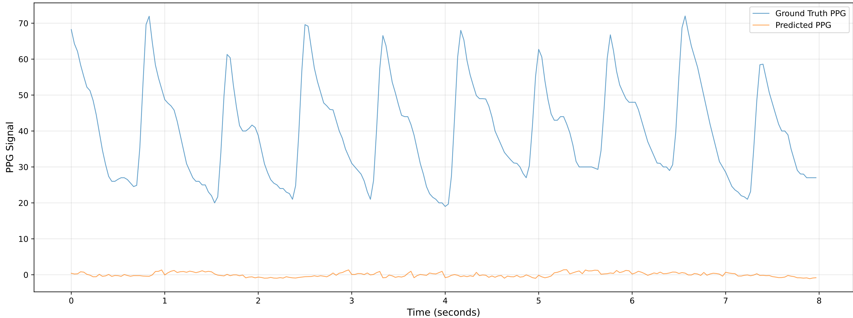
Video 604 - Chunk 2 - Predicted vs Ground Truth PPG
