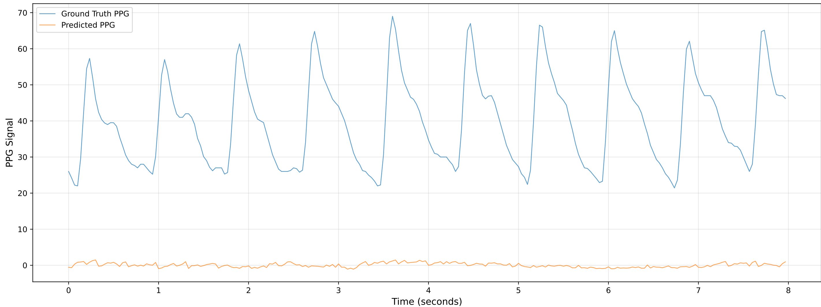
Video 604 - Chunk 3 - Predicted vs Ground Truth PPG
