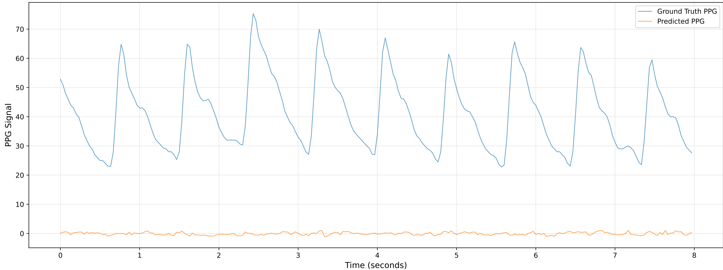
Video 605 - Chunk 1 - Predicted vs Ground Truth PPG
