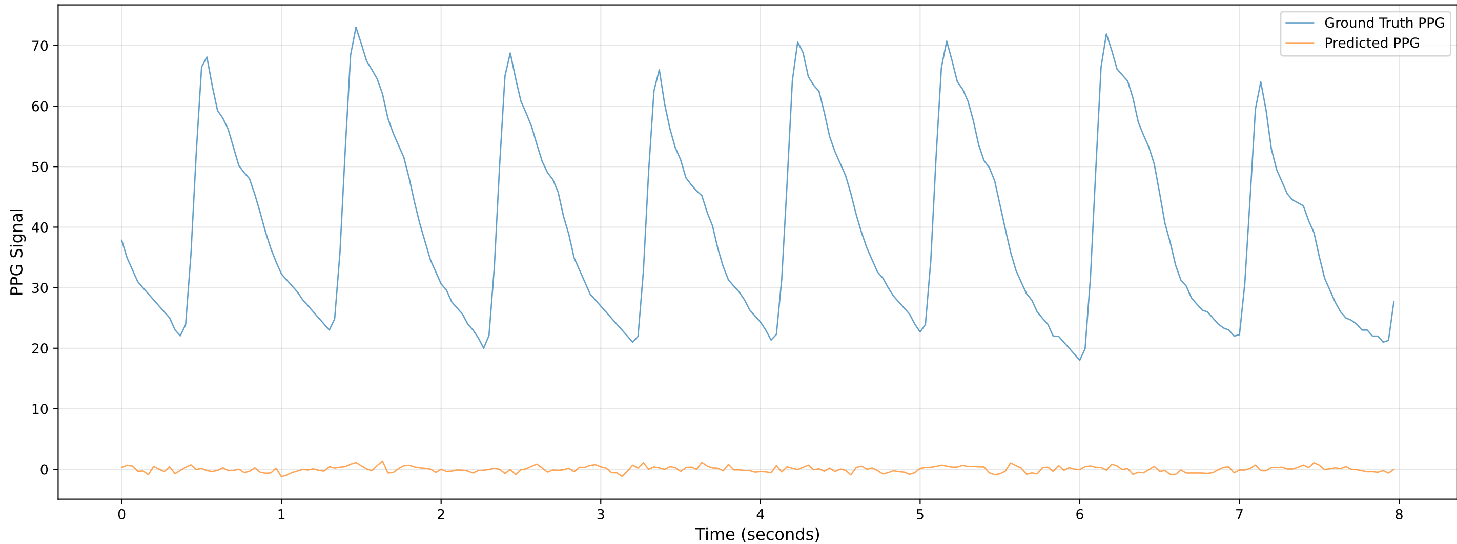
Video 605 - Chunk 6 - Predicted vs Ground Truth PPG
