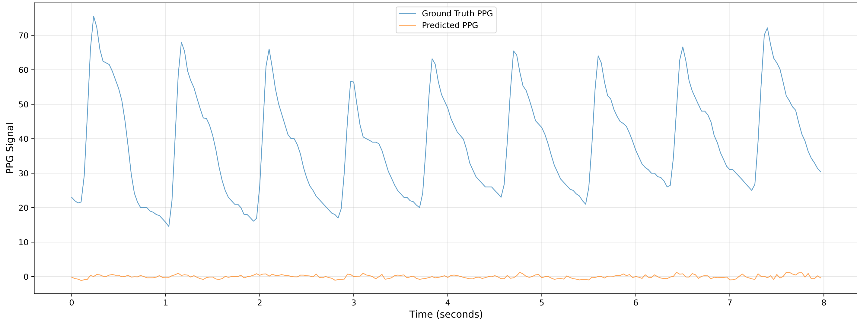
Video 606 - Chunk 7 - Predicted vs Ground Truth PPG
