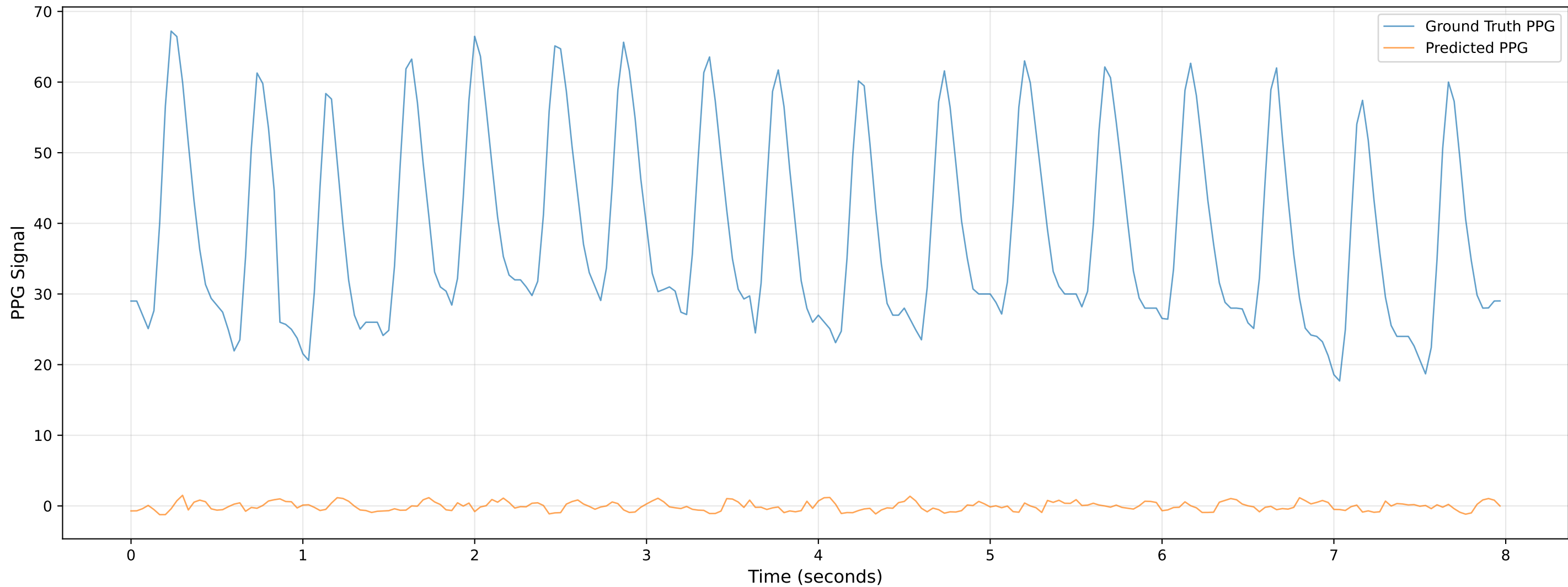
Video 701 - Chunk 1 - Predicted vs Ground Truth PPG
