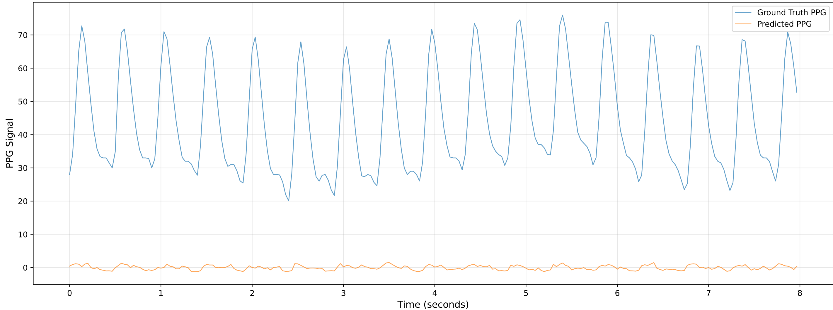
Video 701 - Chunk 7 - Predicted vs Ground Truth PPG
