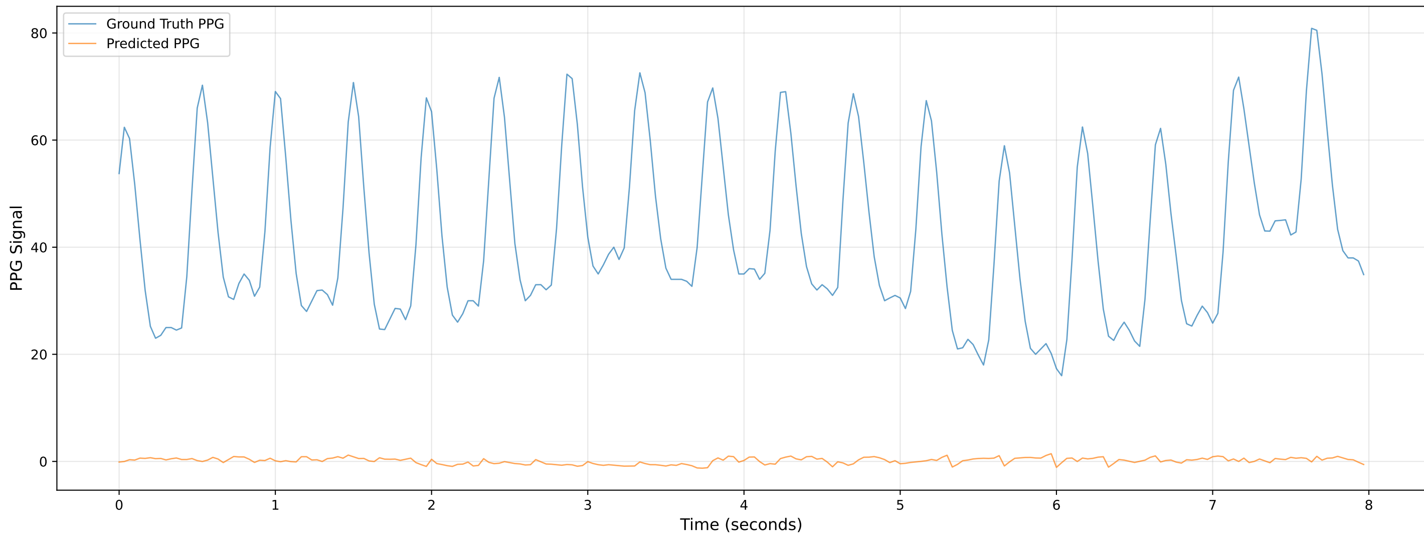
Video 704 - Chunk 7 - Predicted vs Ground Truth PPG
