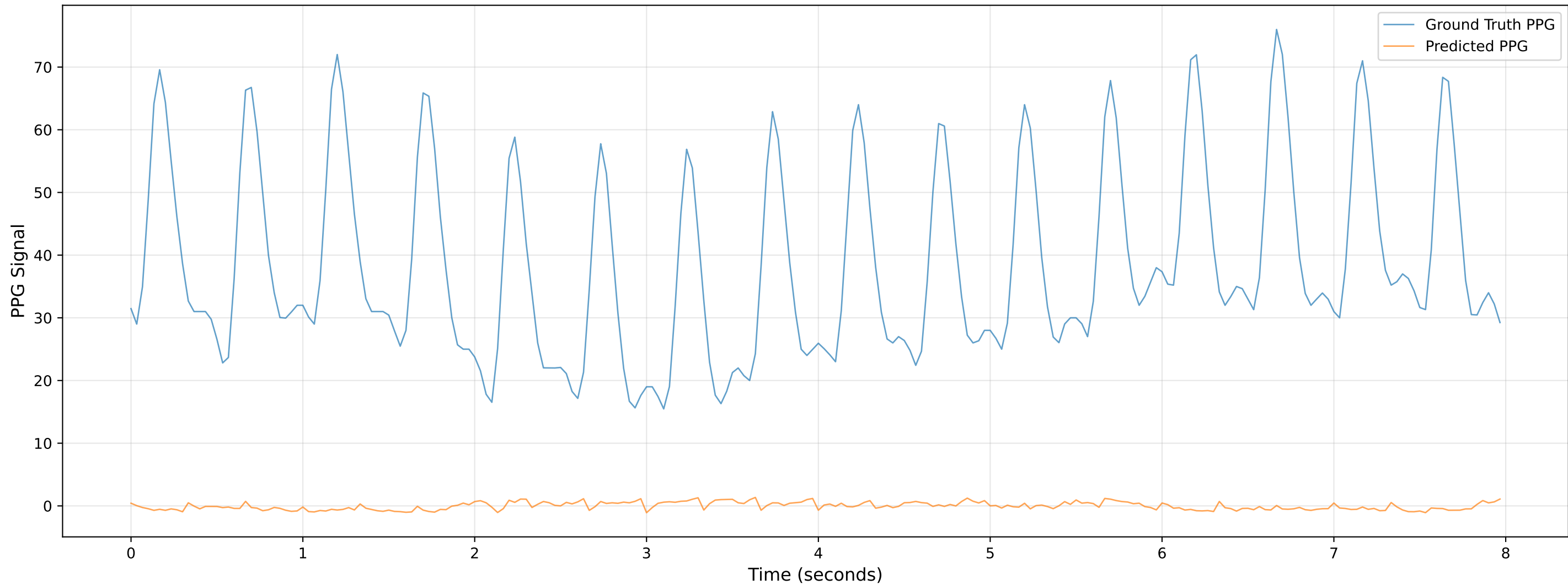
Video 704 - Chunk 8 - Predicted vs Ground Truth PPG
