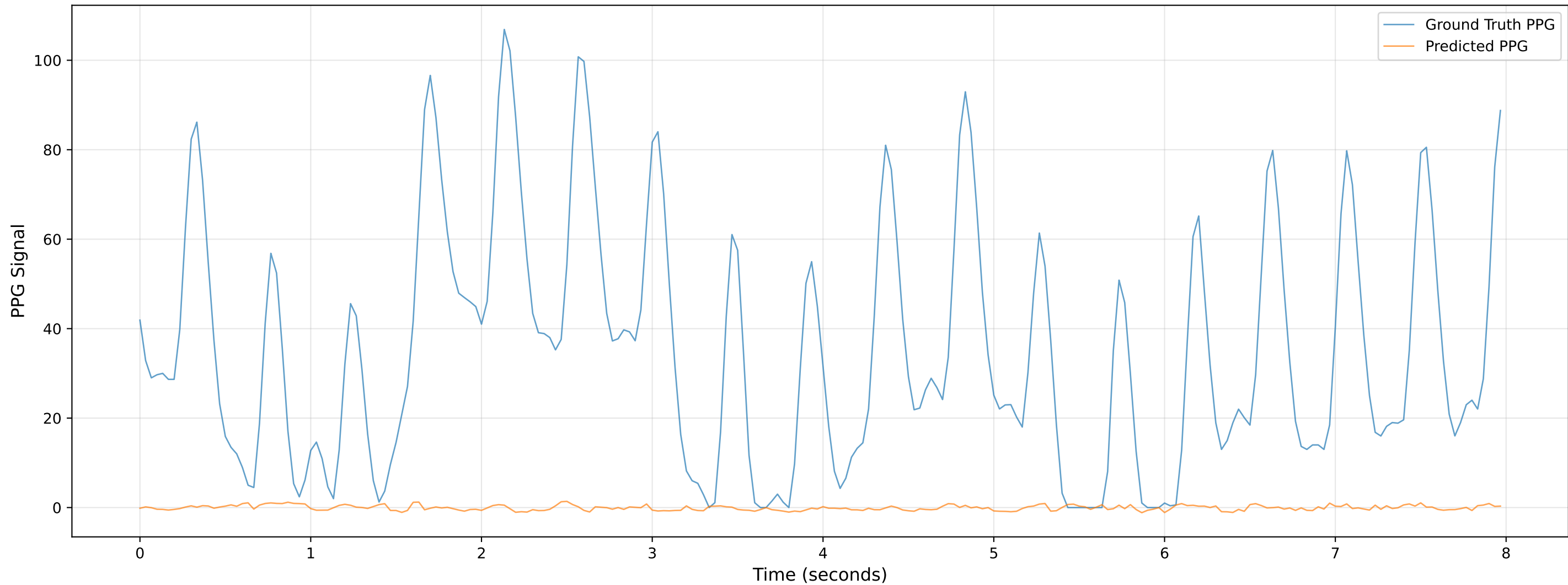
Video 706 - Chunk 4 - Predicted vs Ground Truth PPG
