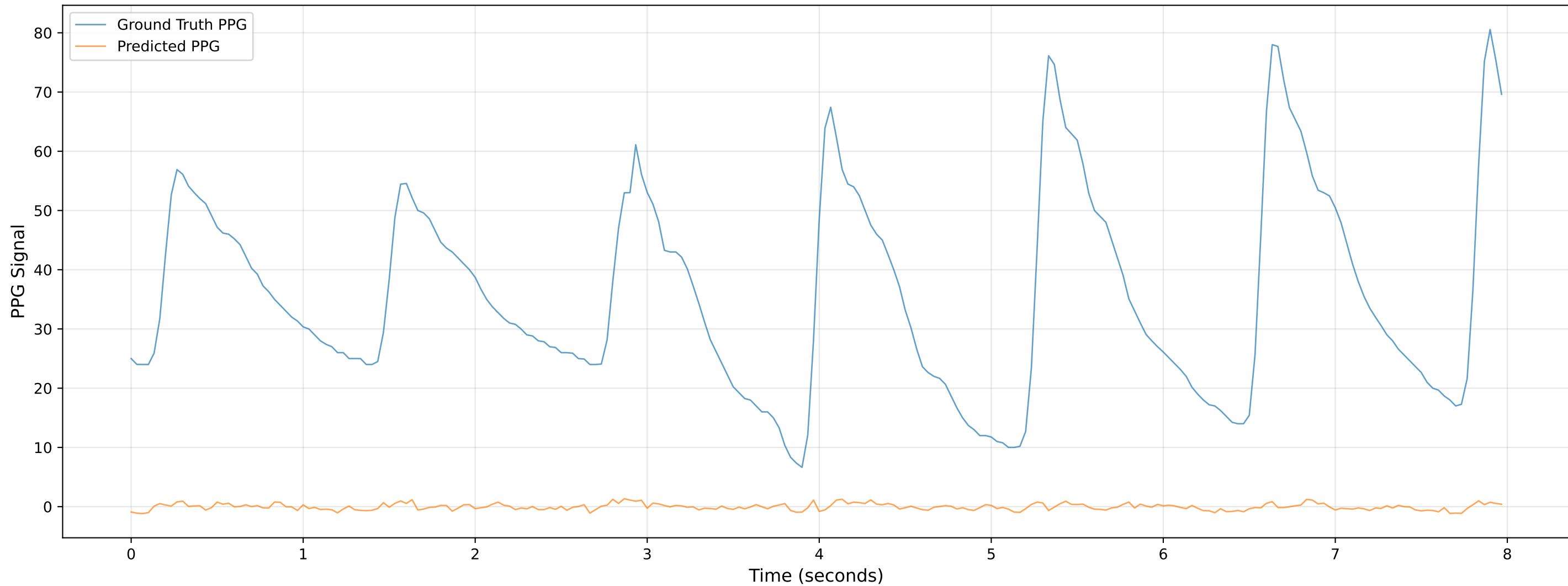
Video 801 - Chunk 0 - Predicted vs Ground Truth PPG
