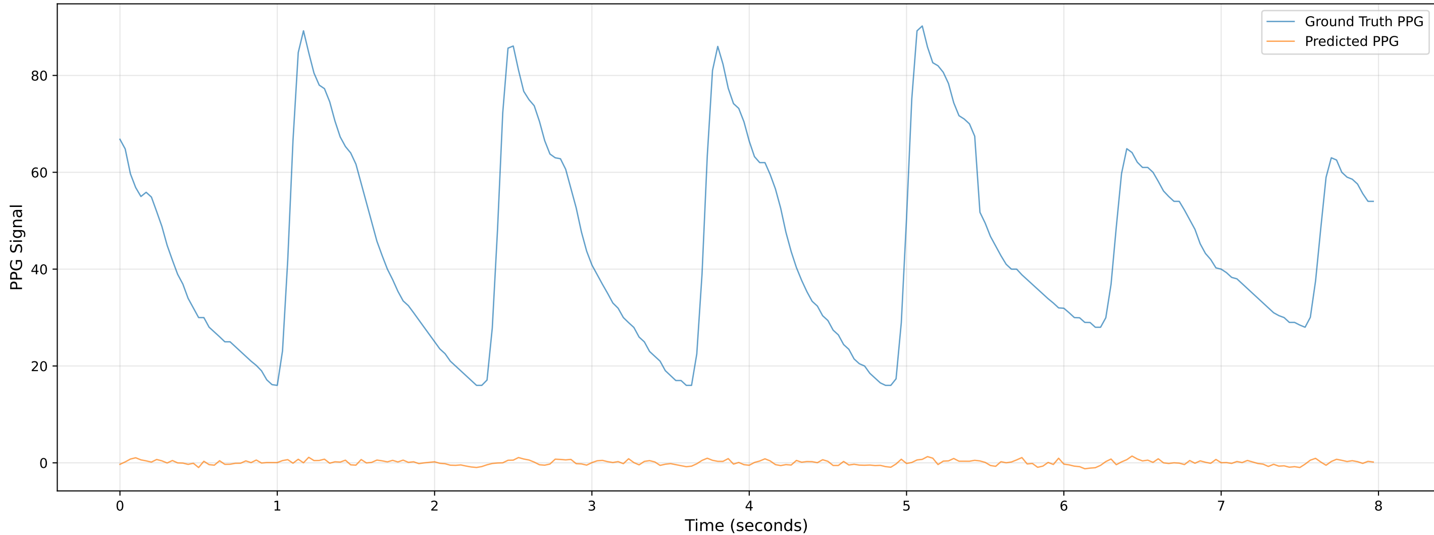
Video 801 - Chunk 1 - Predicted vs Ground Truth PPG
