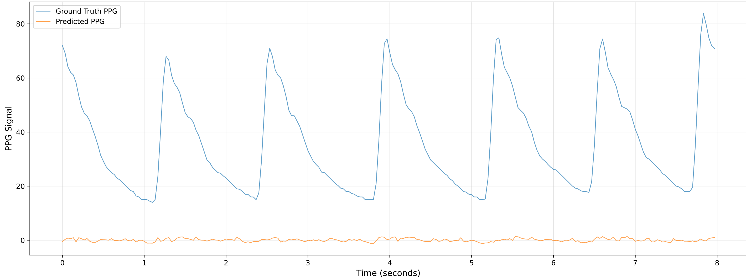
Video 801 - Chunk 5 - Predicted vs Ground Truth PPG
