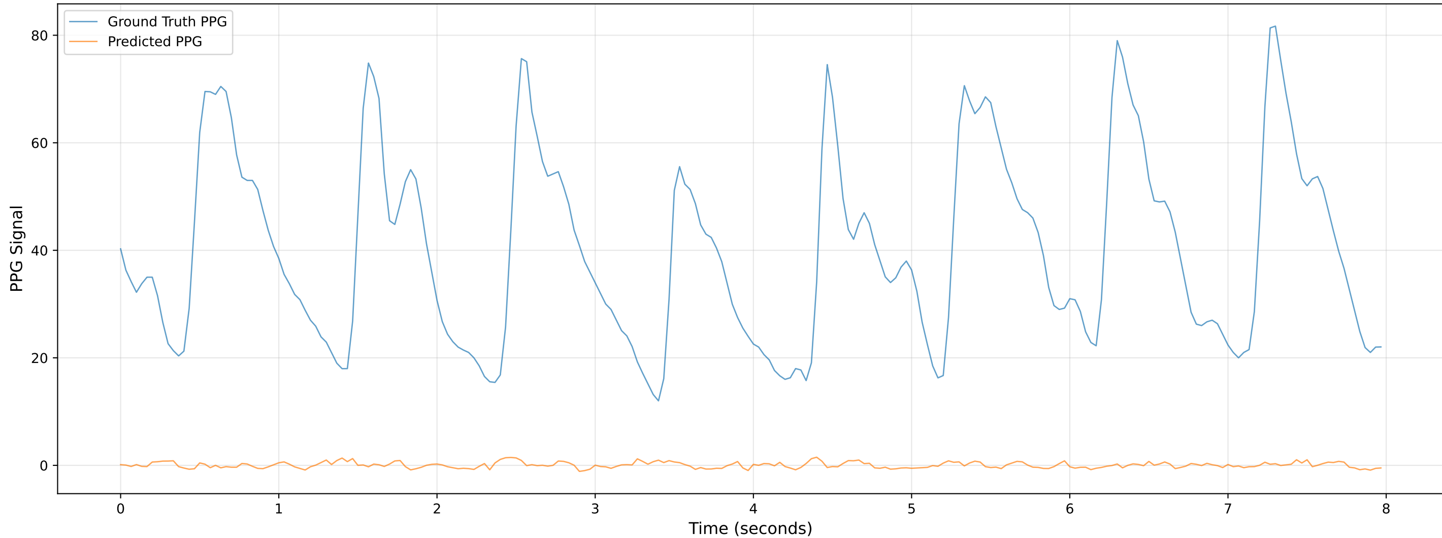
Video 802 - Chunk 6 - Predicted vs Ground Truth PPG
