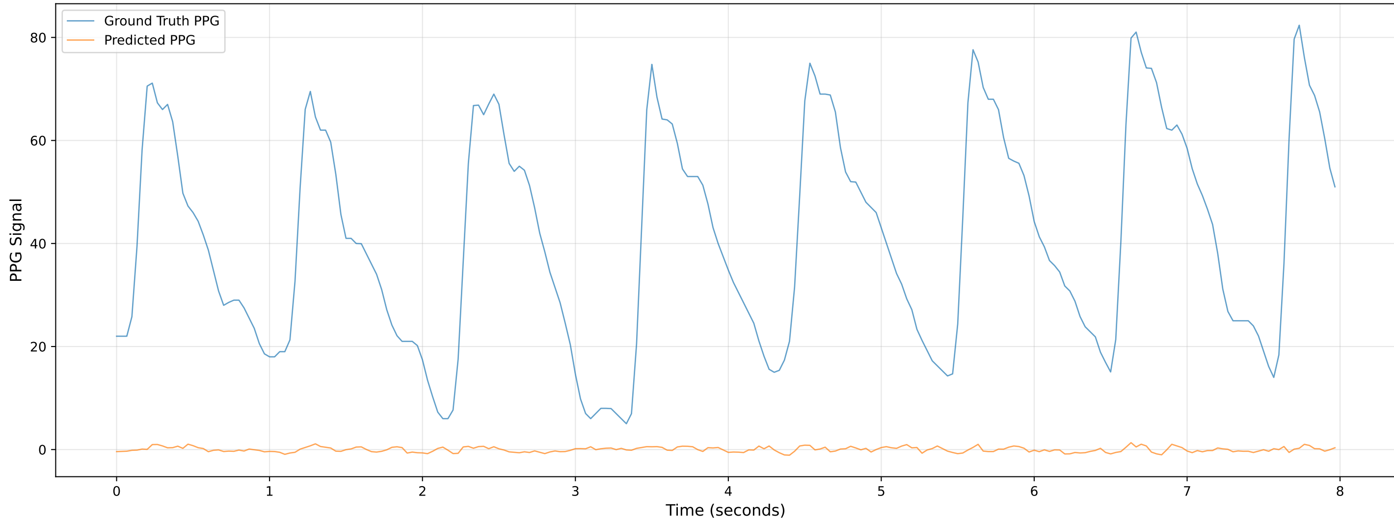
Video 802 - Chunk 7 - Predicted vs Ground Truth PPG
