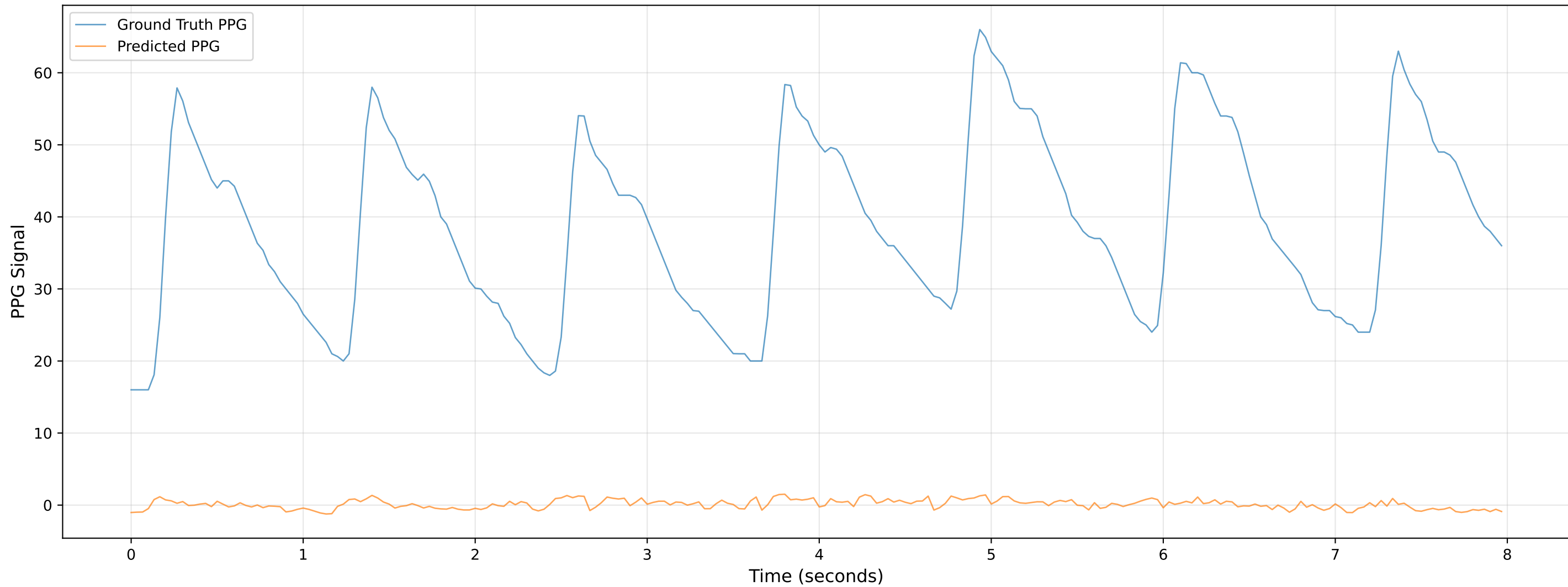
Video 803 - Chunk 1 - Predicted vs Ground Truth PPG
