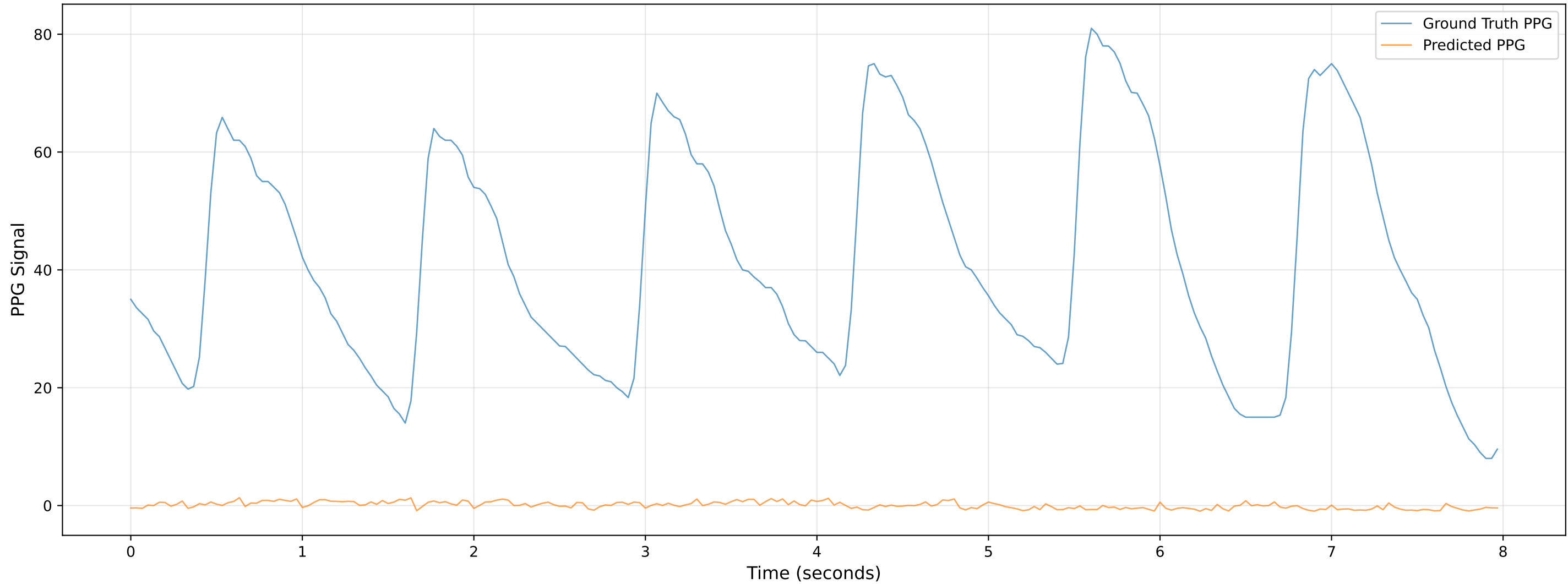
Video 803 - Chunk 4 - Predicted vs Ground Truth PPG
