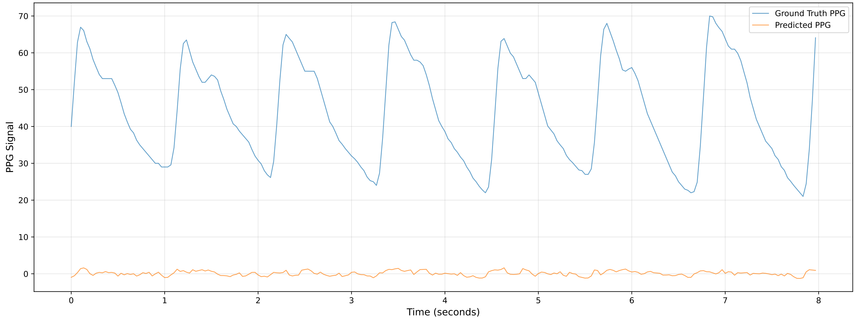
Video 804 - Chunk 0 - Predicted vs Ground Truth PPG
