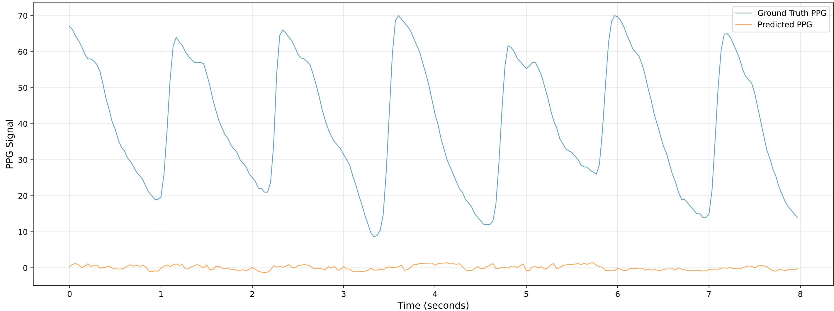
Video 804 - Chunk 1 - Predicted vs Ground Truth PPG
