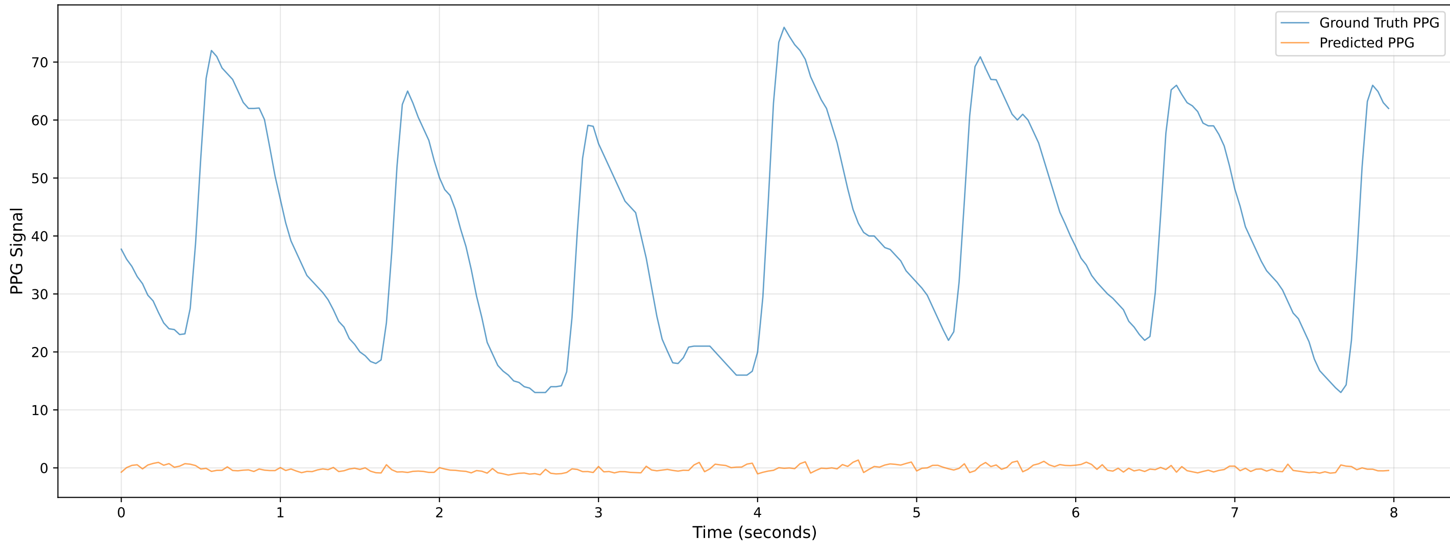
Video 804 - Chunk 3 - Predicted vs Ground Truth PPG
