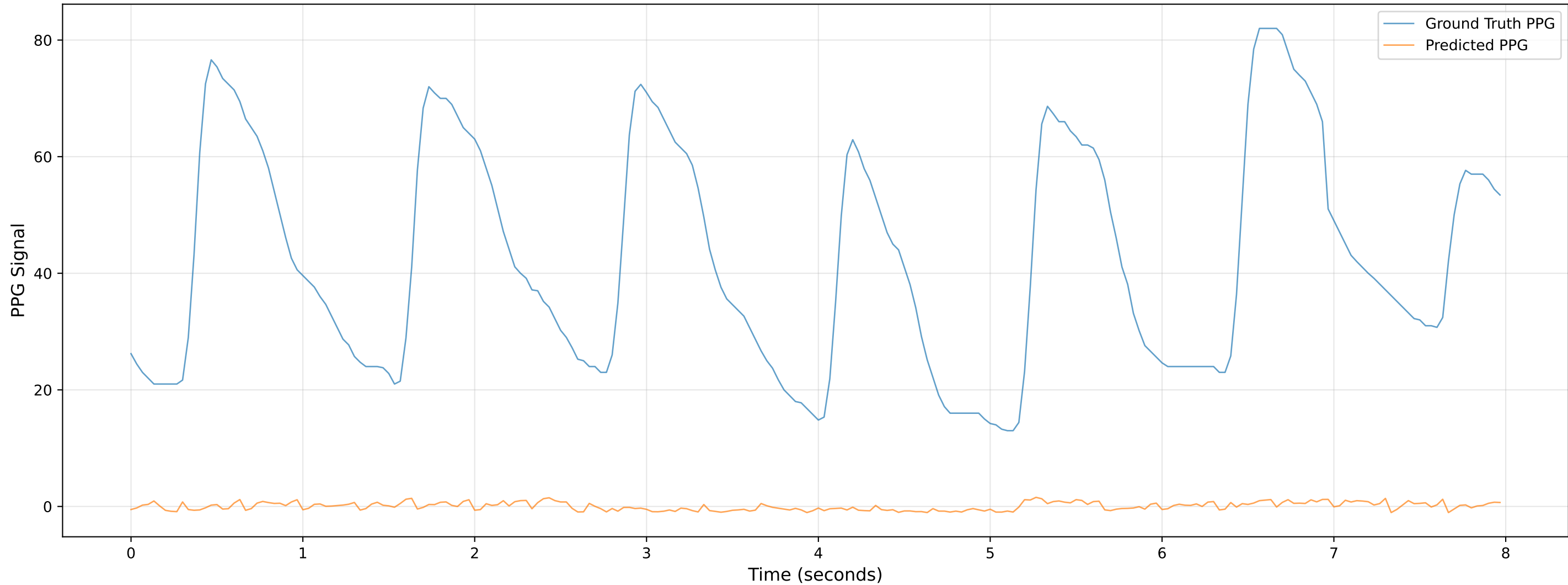
Video 804 - Chunk 5 - Predicted vs Ground Truth PPG
