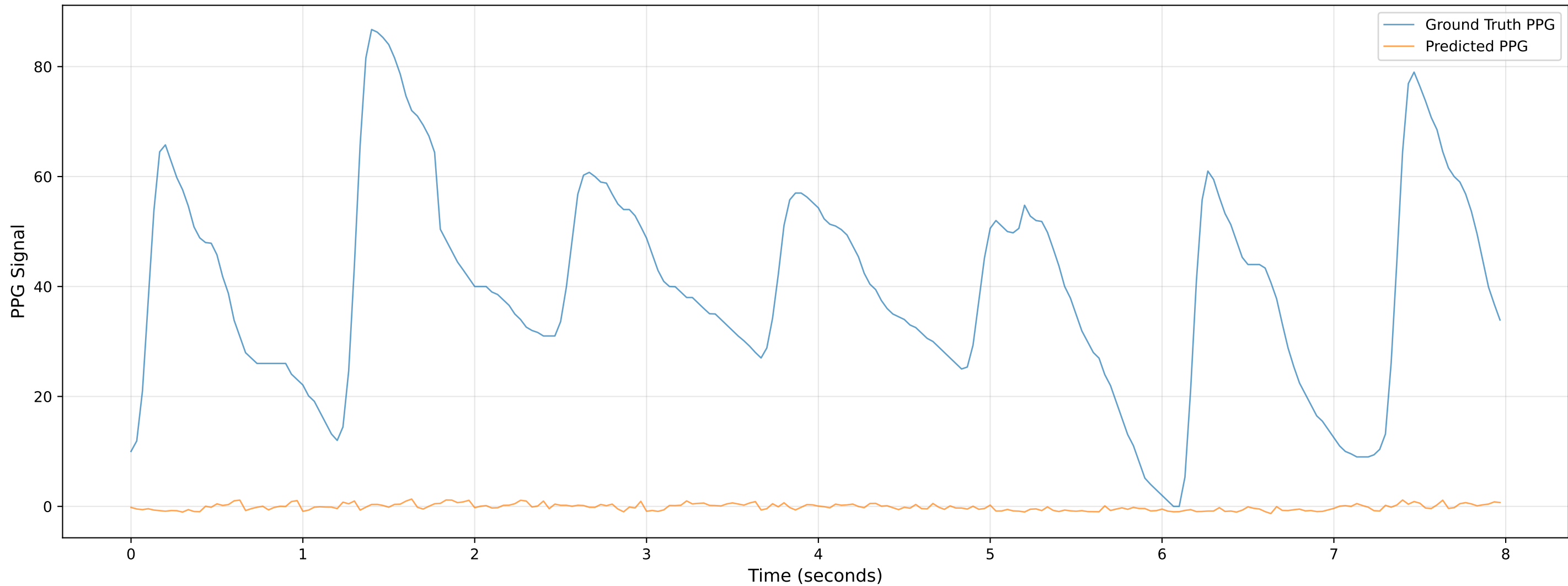
Video 804 - Chunk 7 - Predicted vs Ground Truth PPG
