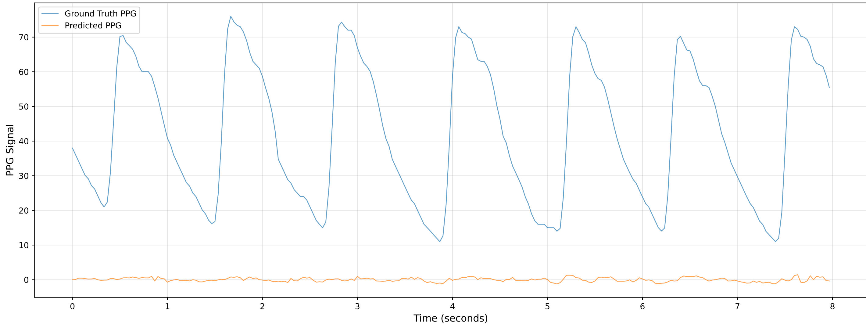
Video 805 - Chunk 0 - Predicted vs Ground Truth PPG
