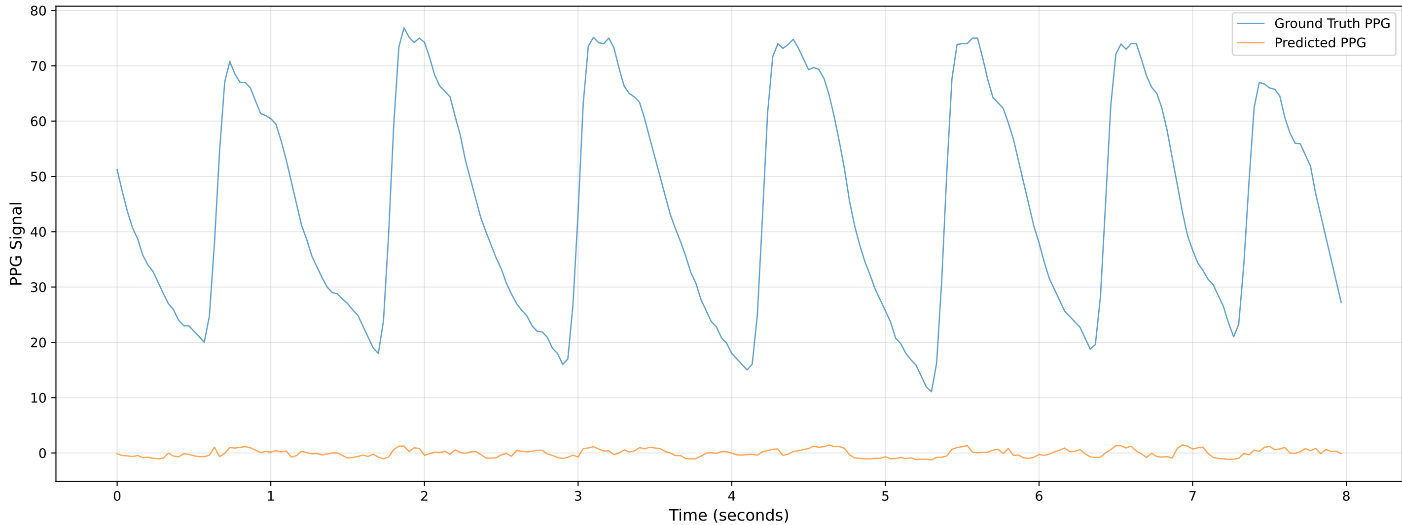
Video 805 - Chunk 5 - Predicted vs Ground Truth PPG
