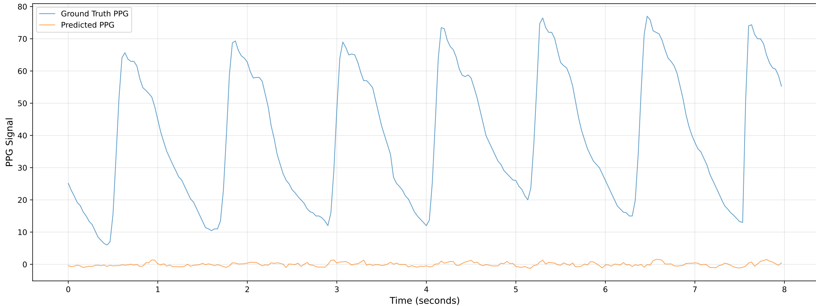
Video 805 - Chunk 6 - Predicted vs Ground Truth PPG
