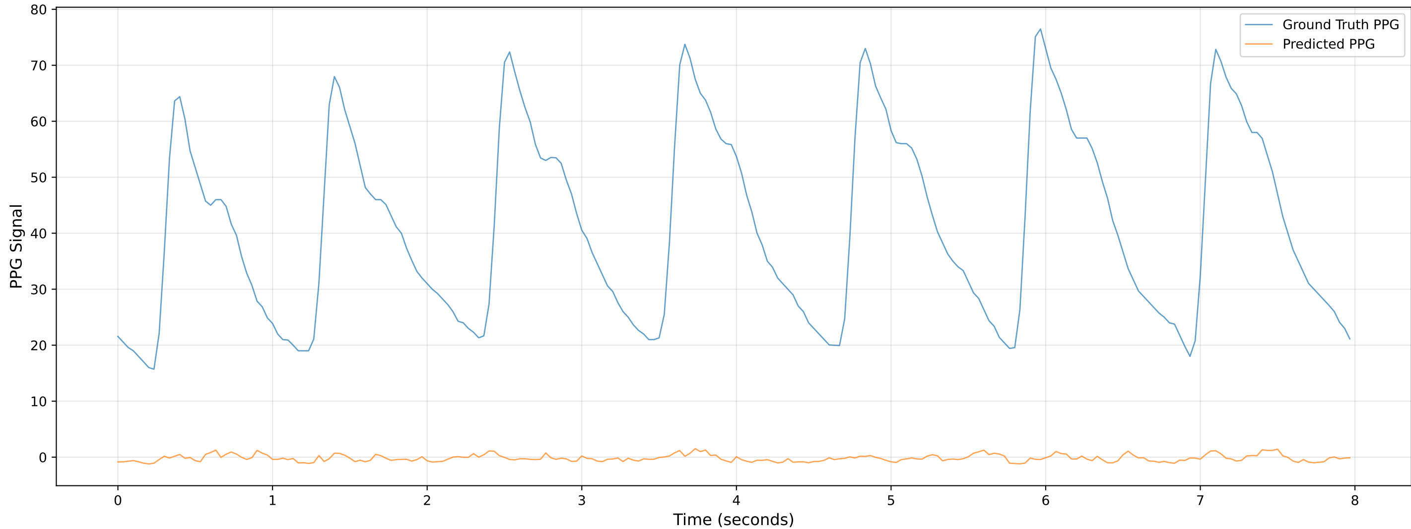
Video 806 - Chunk 1 - Predicted vs Ground Truth PPG
