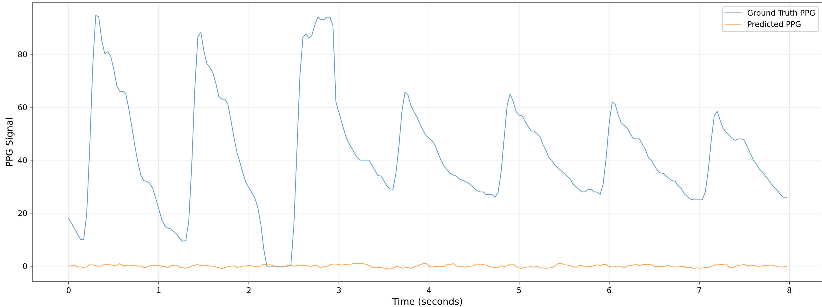
Video 902 - Chunk 4 - Predicted vs Ground Truth PPG
