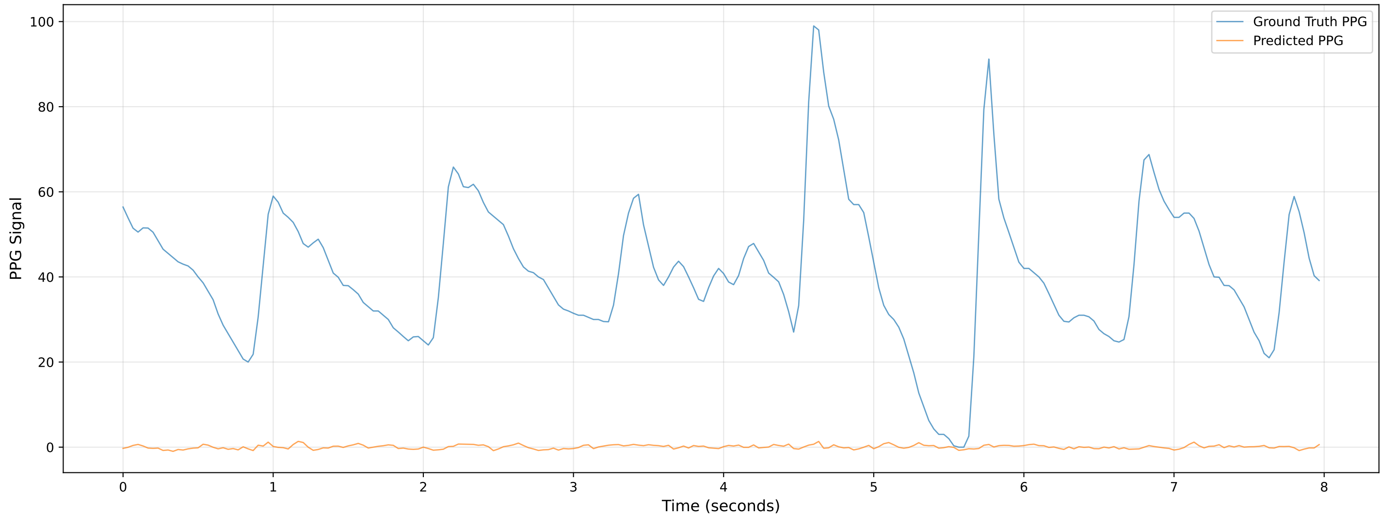
Video 902 - Chunk 6 - Predicted vs Ground Truth PPG
