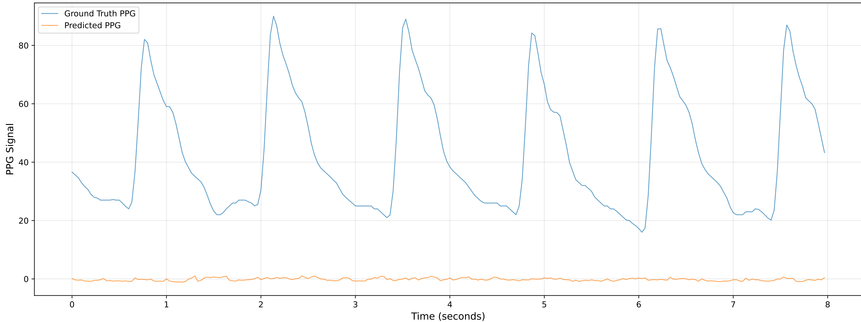
Video 904 - Chunk 3 - Predicted vs Ground Truth PPG
