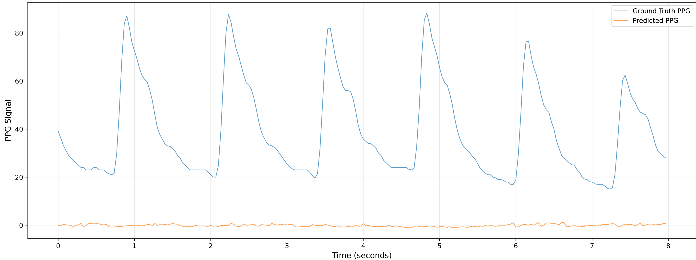
Video 904 - Chunk 4 - Predicted vs Ground Truth PPG
