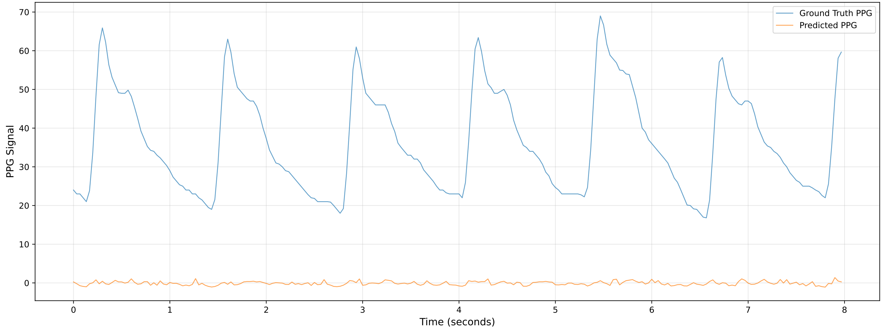
Video 906 - Chunk 0 - Predicted vs Ground Truth PPG
