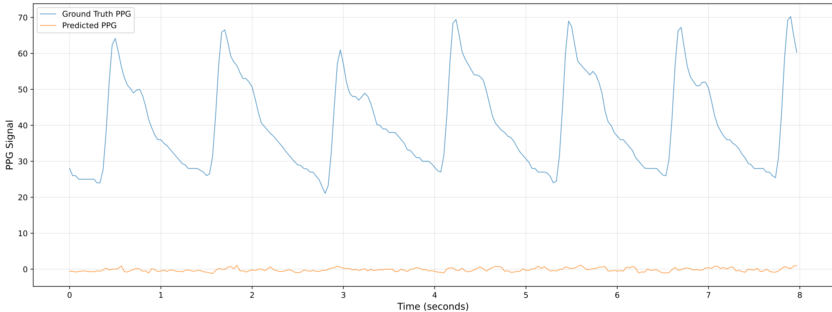
Video 906 - Chunk 3 - Predicted vs Ground Truth PPG
