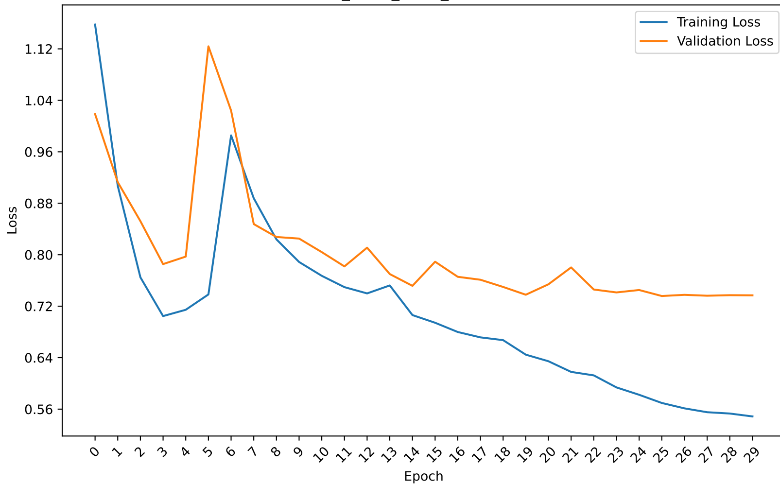
UBFC_UBFC_PURE_tscan Losses
