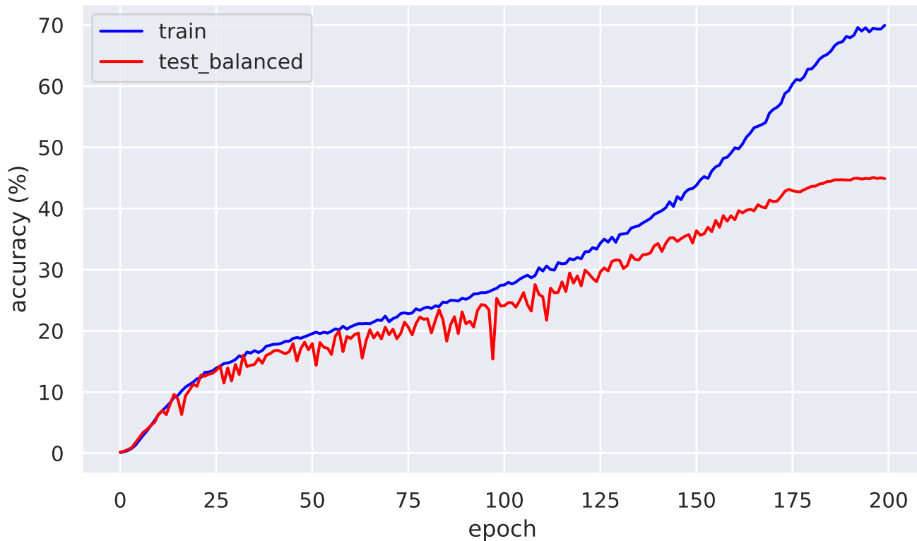
Average accuracy over classes at each epoch
