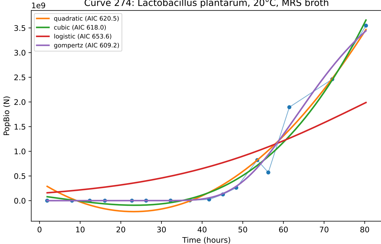
Curve 274: Lactobacillus plantarum , 20°C, MRS broth
