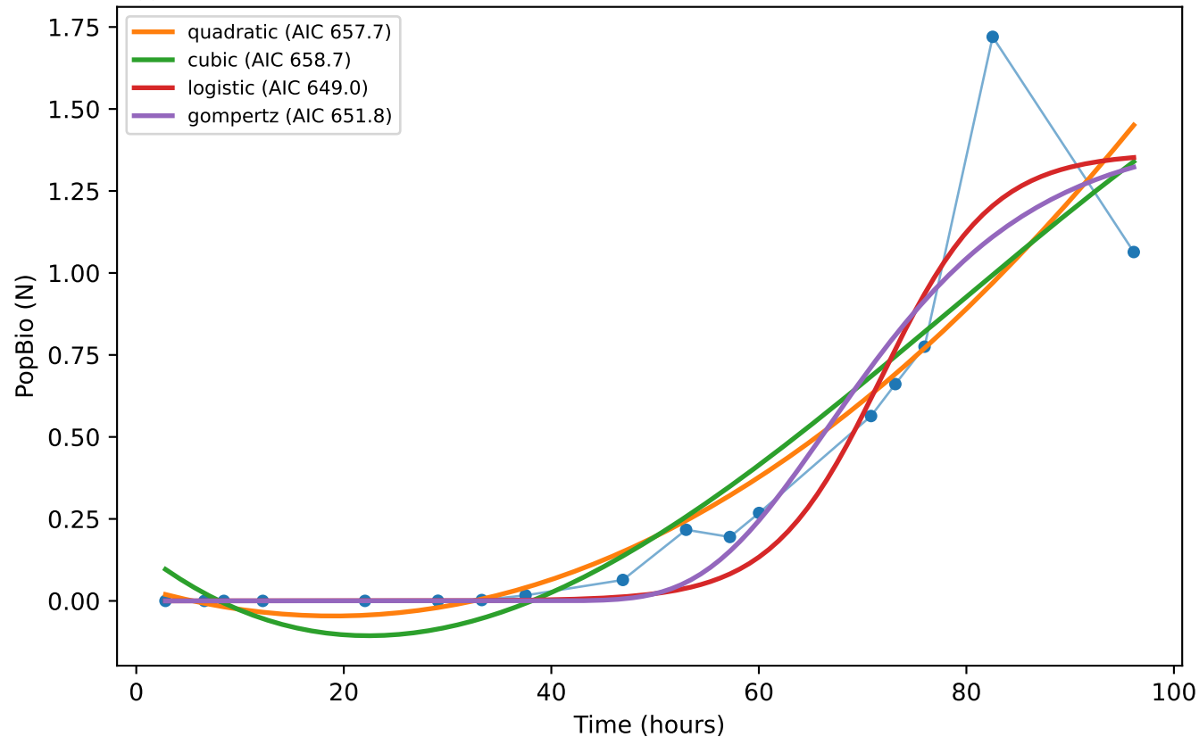
1e9 Curve 279: Weissella viridescens , 16°C, MRS broth
