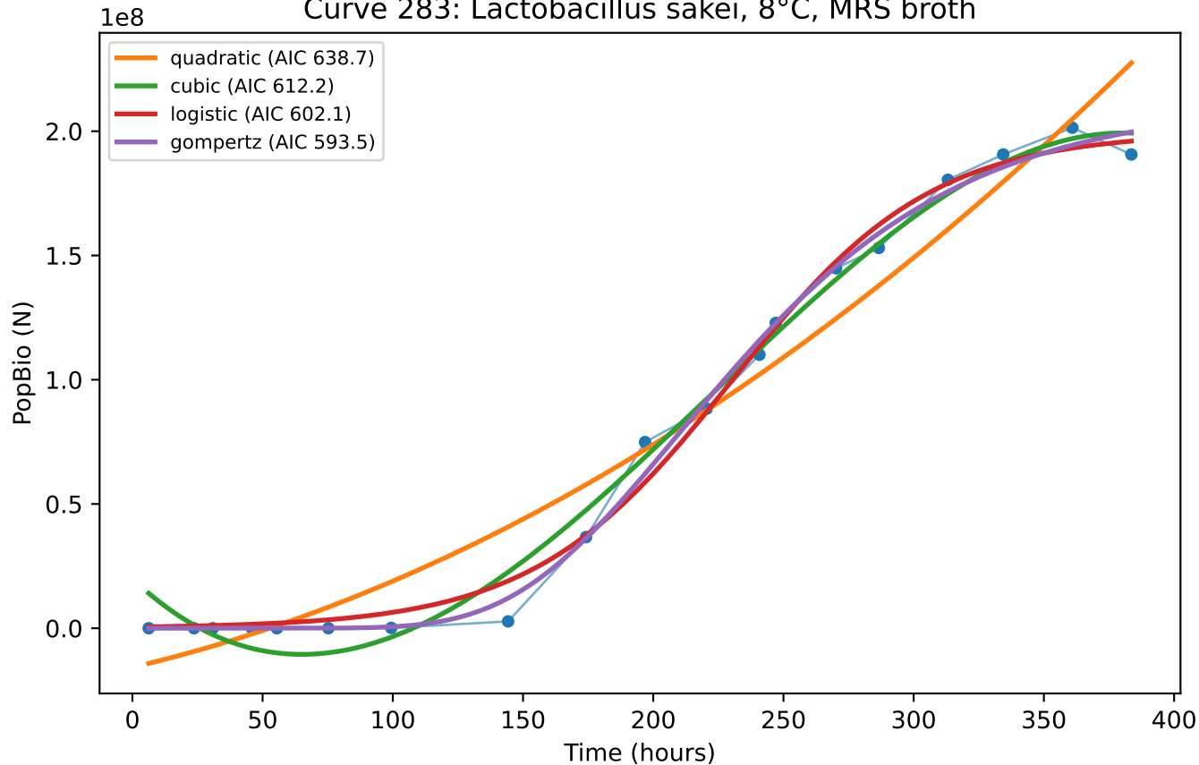
Curve 283: Lactobacillus sakei , 8°C, MRS broth
