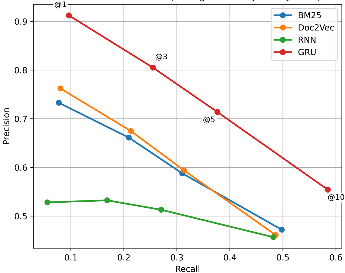
Precision-Recall Curve (Dialogue History - Only User)
