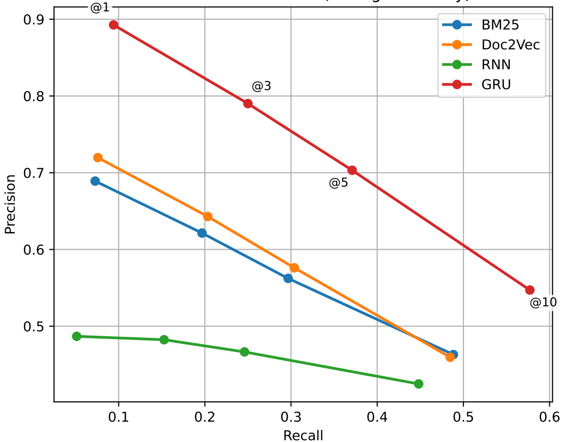
Precision-Recall Curve (Dialogue History)
