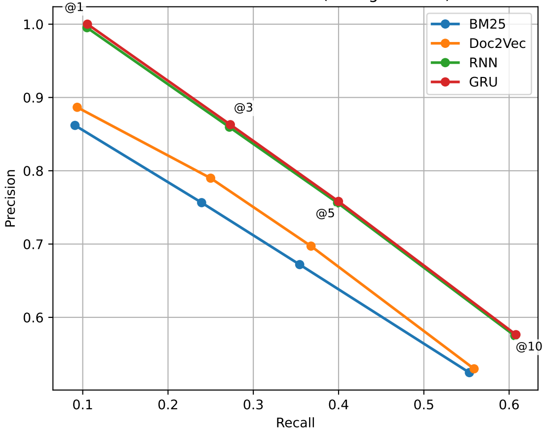
Precision-Recall Curve (Dialogue State)
