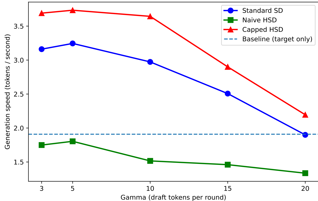
Speculative decoding speed vs draft length
