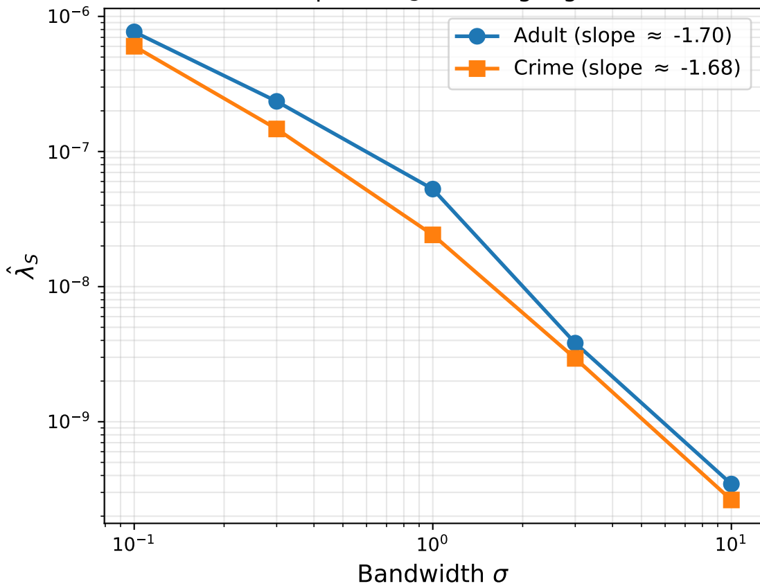
Empirical \hat{\lambda}_S vs \sigma (log-log)
