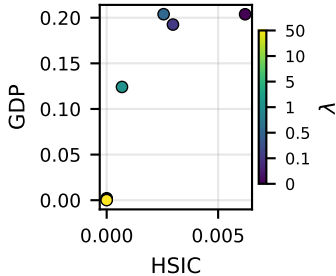
(c) GDP vs. HSIC (Thm. 3.4)
