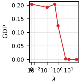
(a) GDP vs. \lambda
