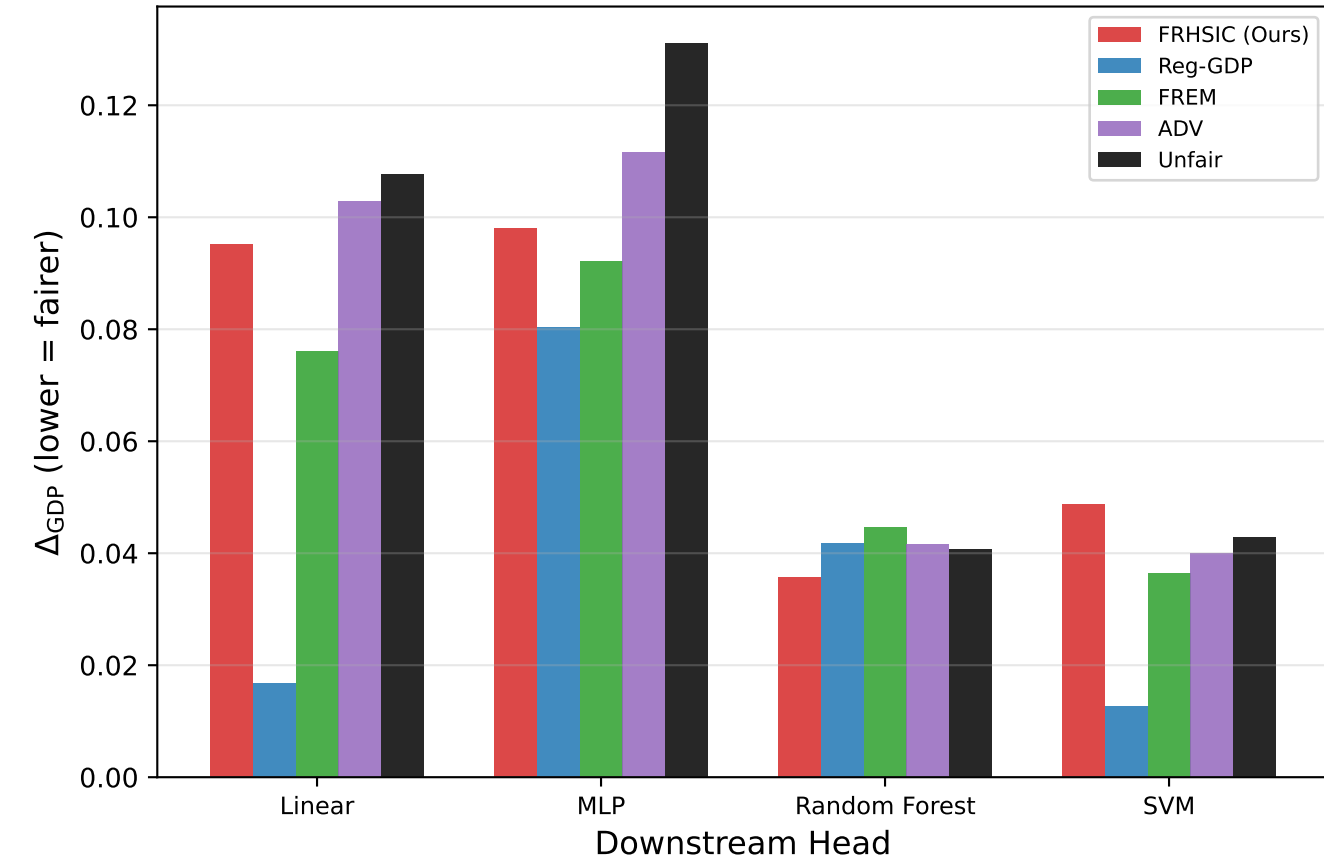
COMPAS
