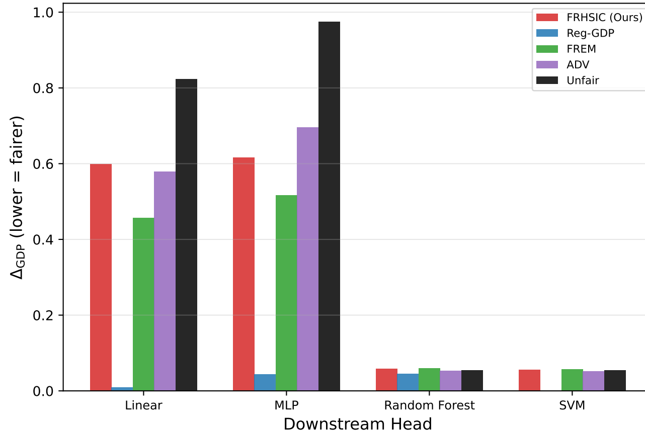
ADULT
