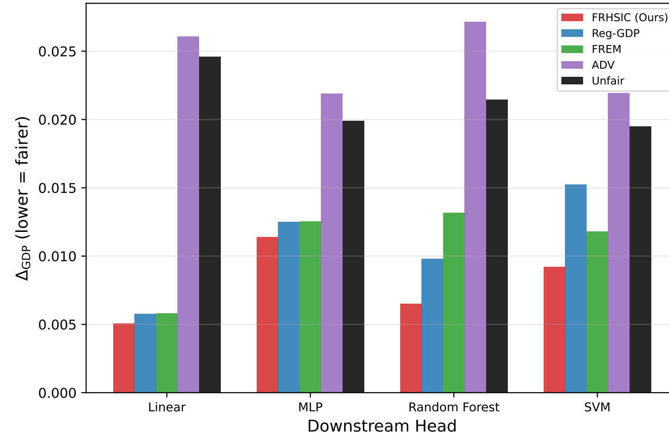
COMMUNITIES
