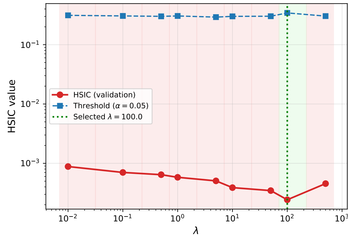
COMPAS
