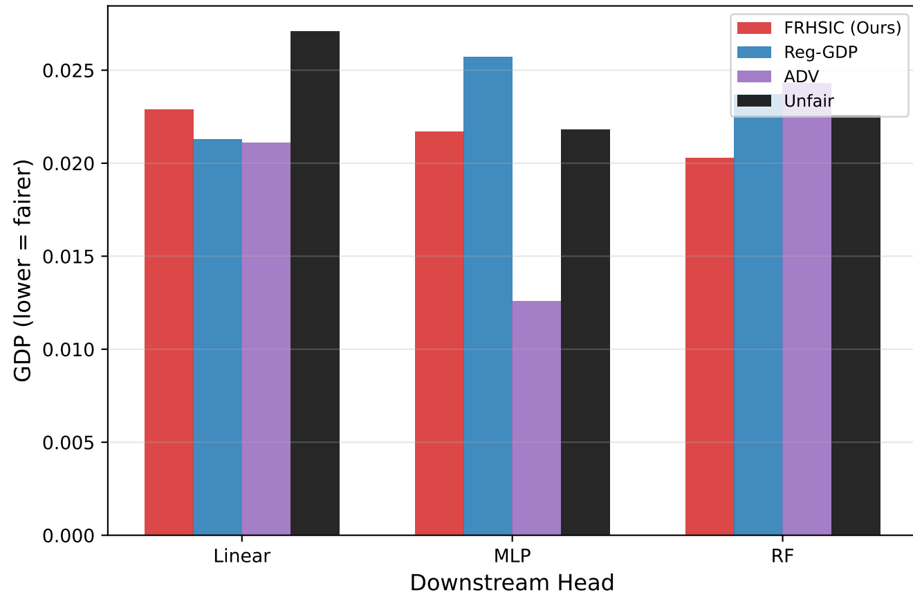
Crime ( \lambda = 100 )
