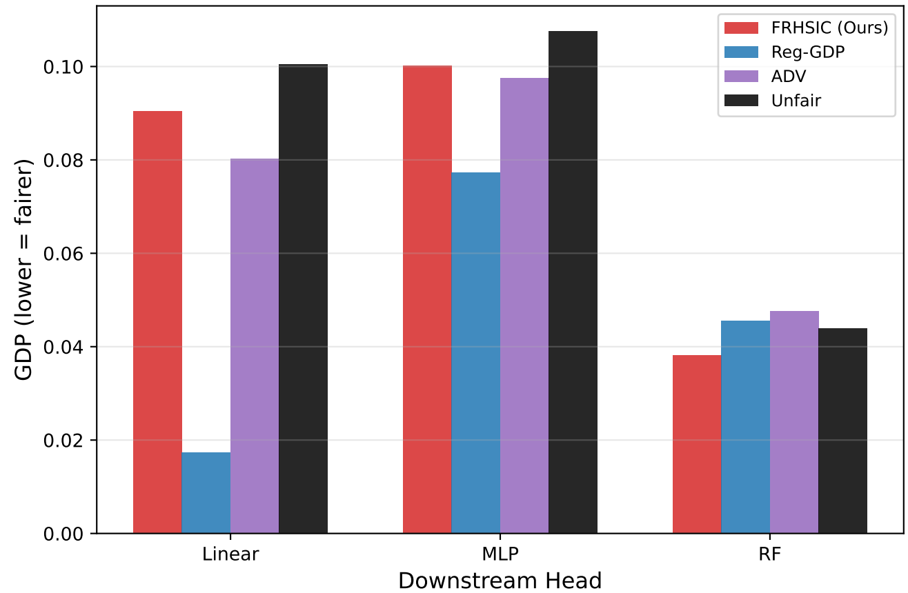
COMPAS ( \lambda = 100 )
