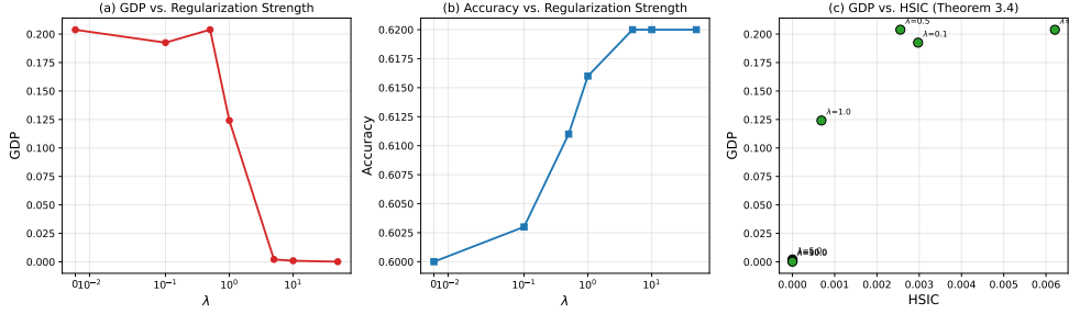
FIG. 2. Synthetic experiment results. (a) GDP decreases as \lambda increases. (b) Accuracy remains stable across regularization strengths. (c) GDP vs. HSIC shows a monotone relationship, consistent with the conditional-gap-control interpretation of Theorem 3.4 (the plot displays monotonic dependence, not the LHS/RHS of the bound). The in-image panel label refers to the same result under the prior numbering (“Theorem 2”); the corresponding statement in the current numbering is Theorem 3.4. The overlapping \lambda tick labels in panel (a) will be regenerated for camera-ready.
