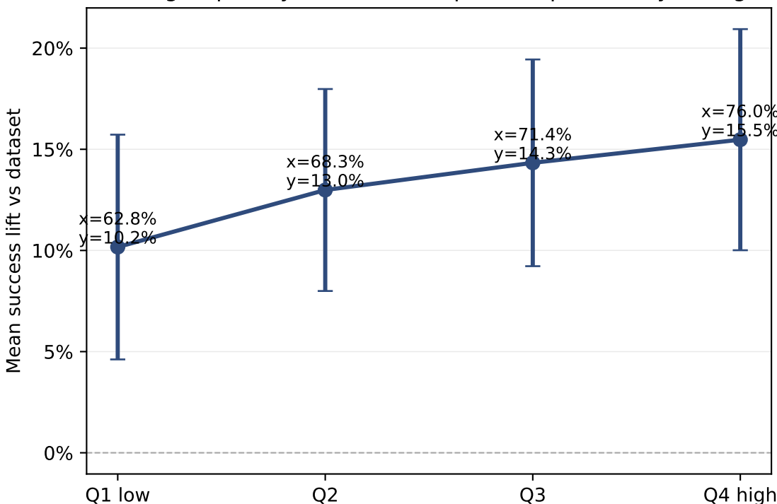
train: grouped by Fraction with positive probability change
